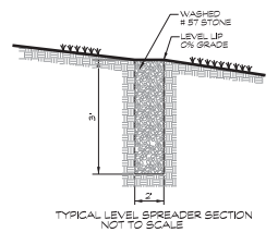
TYPICAL LEVEL SPREADER SECTION NOT TO SCALE
